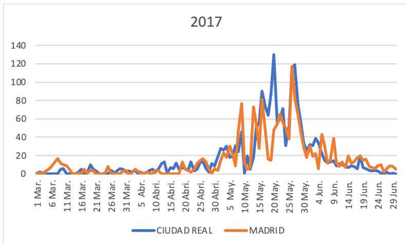
Figure 3. Grains of grass pollen per cubic meter of air.
